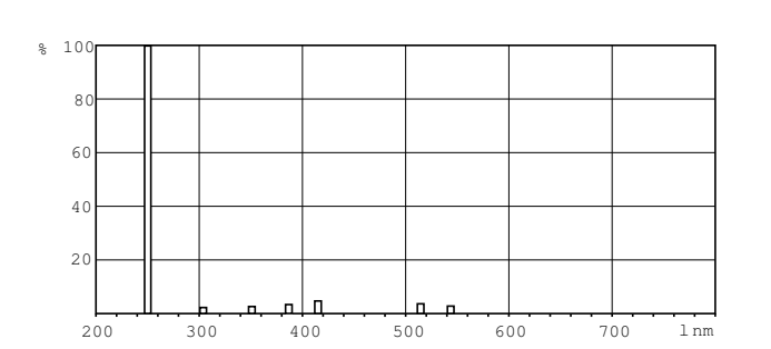
XDPB_XUTUVTLD-Spectral power distribution B/W
